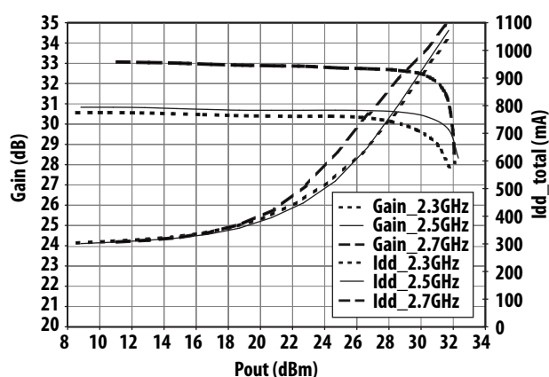
Figure 13. CW Gain vs Pout @ 85°C high-gain mode, Vdd = 5V
