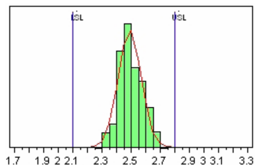
Figure 1c. Vc Distribution for I_q(\text{total})=240\text{mA}
